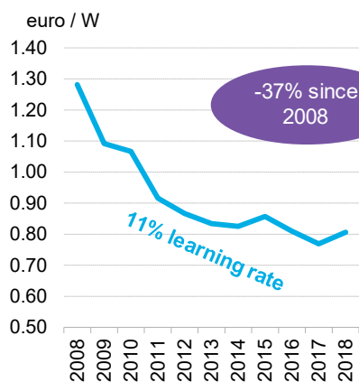
Figure 4: Technology cost reductions in solar PV, onshore wind and lithium-ion batteries
